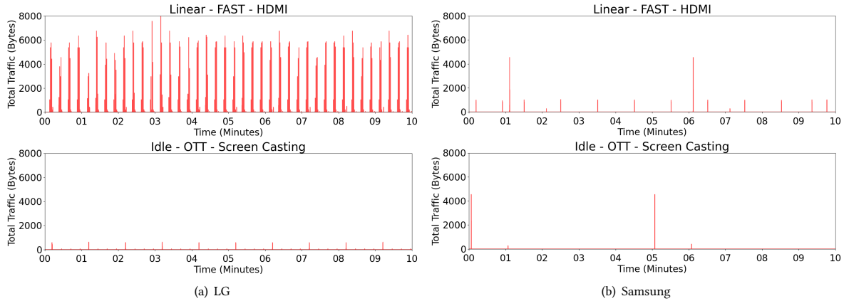
Figure 6: 10 minutes of ACR traffic in different scenarios during LIn-OIn in US.
